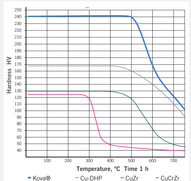
Kova softening behavior - resistance against softening
