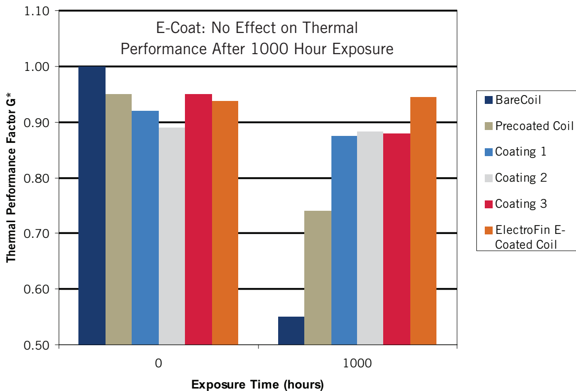
Thermal Performance After 1000 Hour Prohesion Test
